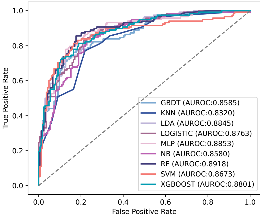
ROC Curves of Multiple Models
